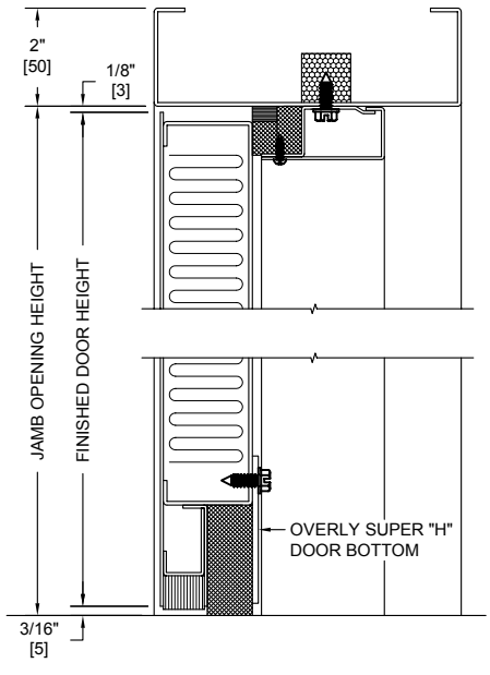
VERTICAL SECTION
