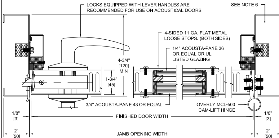
HORIZONTAL SECTION
