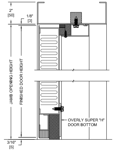
VERTICAL SECTION
