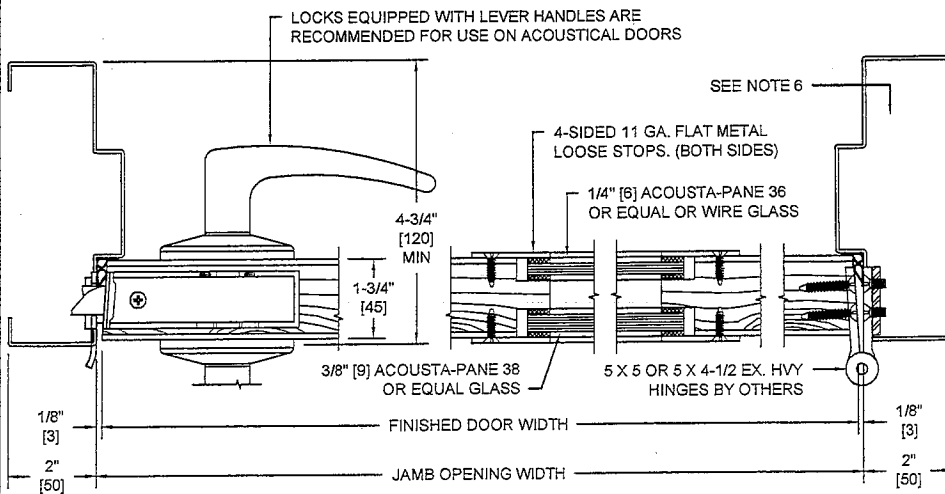
HORIZONTAL SECTION
