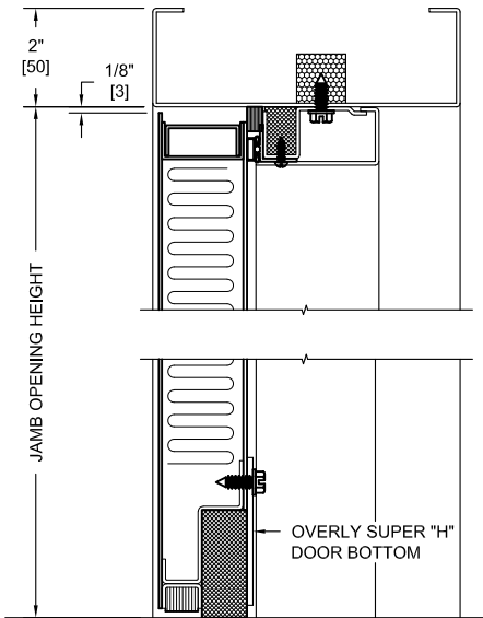
VERTICAL SECTION
