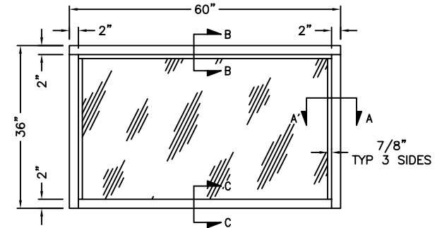
ELEVATION VIEW
