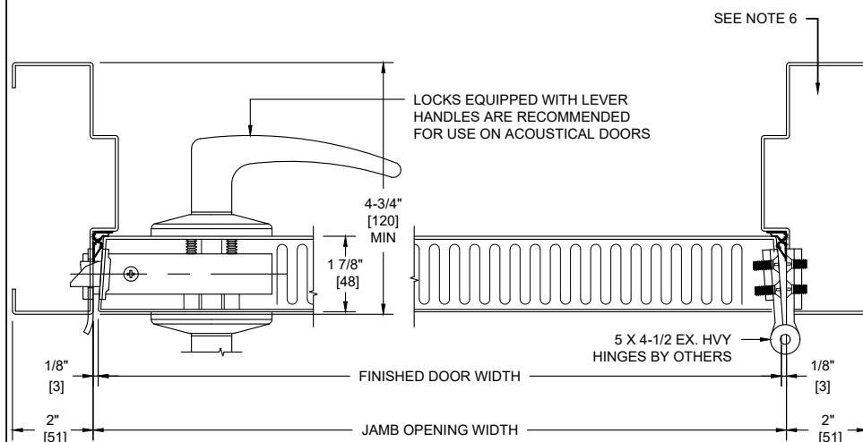
HORIZONTAL SECTION
