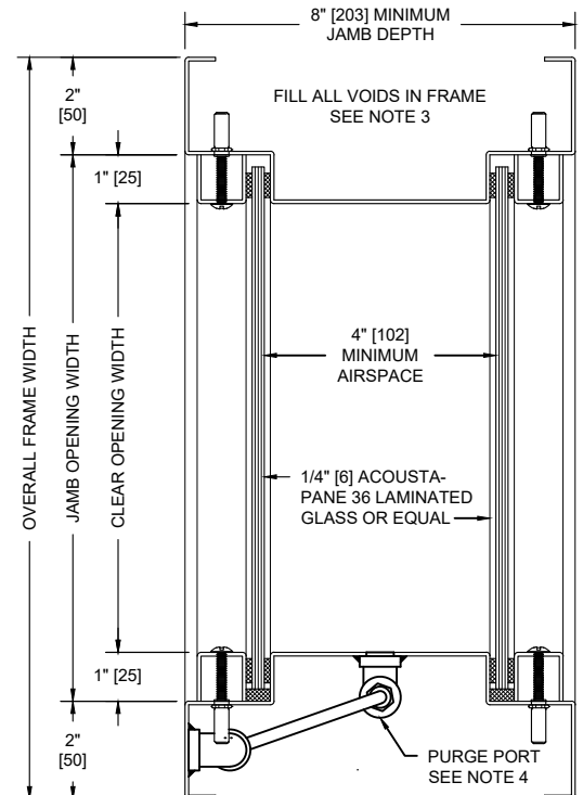
VERTICAL SECTION
