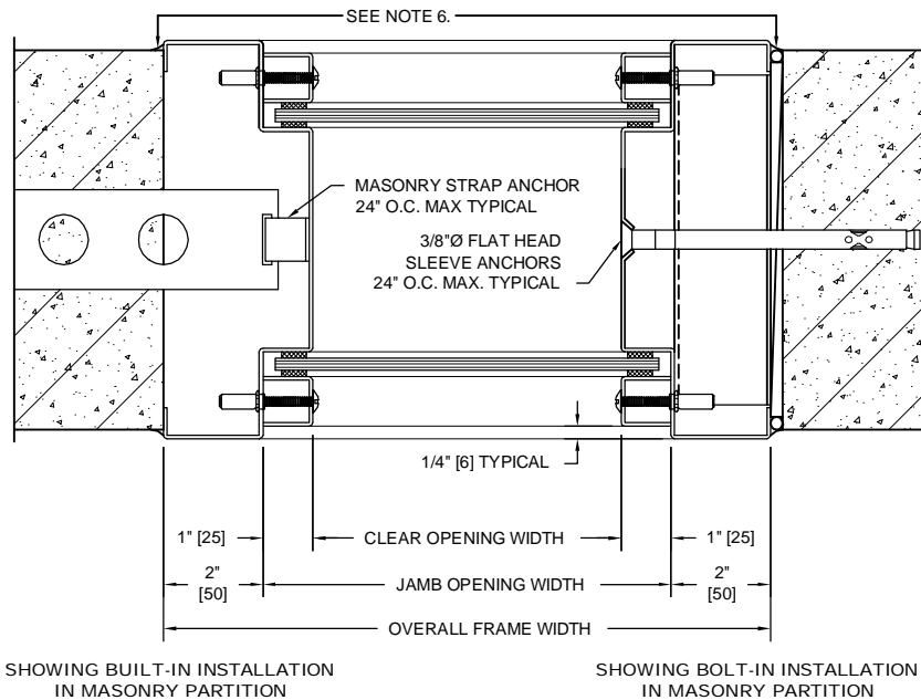
HORIZONTAL SECTION
