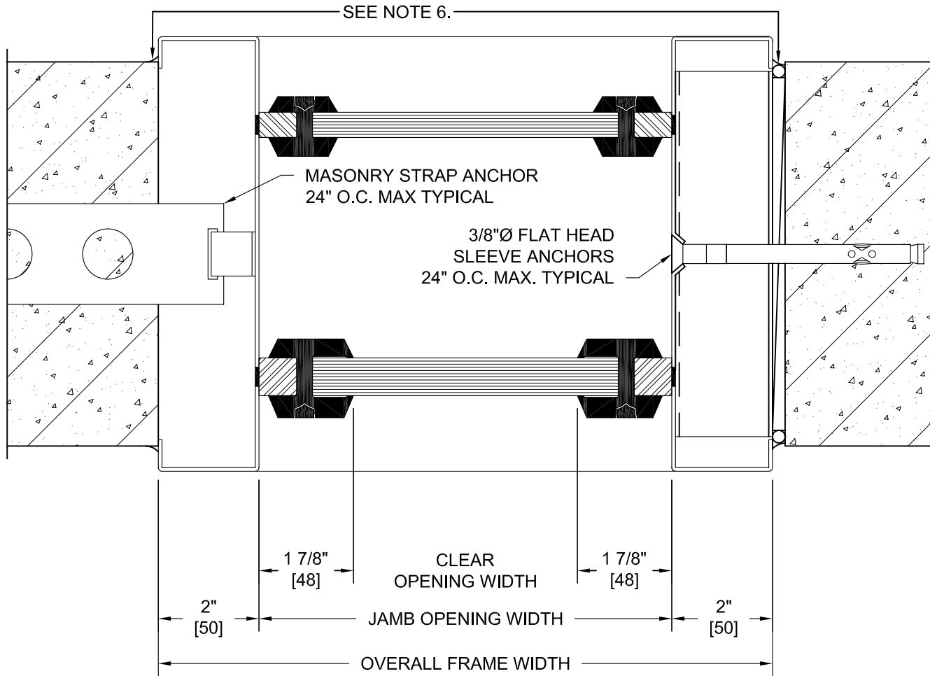
SHOWING BUILT-IN INSTALLATION IN MASONRY PARTITION
