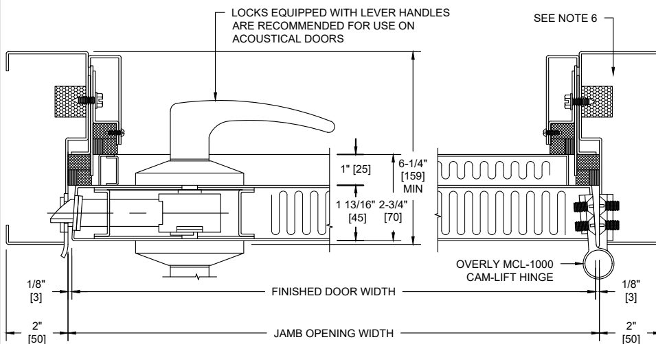
HORIZONTAL SECTION
