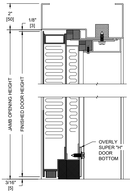
VERTICAL SECTION
