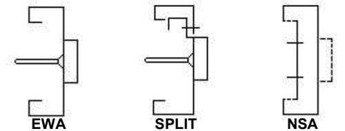
EWA EXISTING WALL ANCHOR SPLIT SPLIT FRAME NSA NEW STUD WALL ANCHOR
