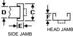
FRAME PROFILE
