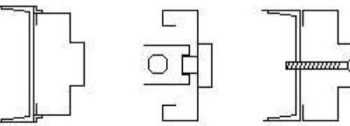
CF-WLD WELD-IN FRAME NMA NEW MASONRY ANCHOR CF-BLT BOLT-IN CHANNEL IRON
