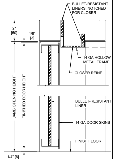
VERTICAL SECTION
