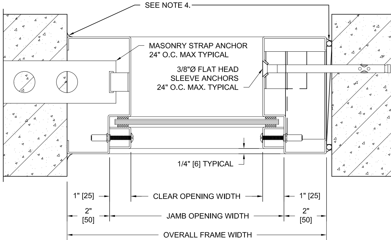
SHOWING BUILT-IN INSTALLATION IN MASONRY PARTITION
