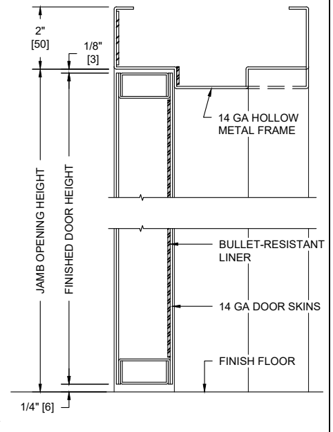
VERTICAL SECTION
