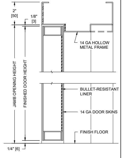
VERTICAL SECTION
