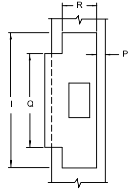
STRIKE DETAIL
