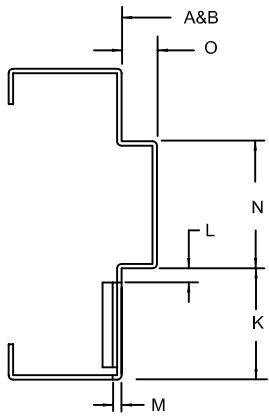
FRAME PROFILE
