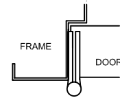
DOUBLE MORTISE
