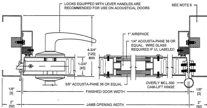
HORIZONTAL SECTION
