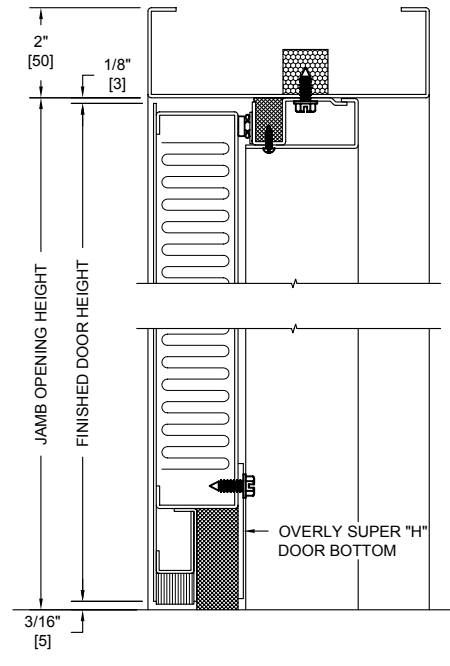
VERTICAL SECTION
