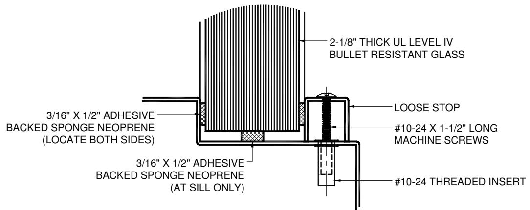
DETAIL "A"
